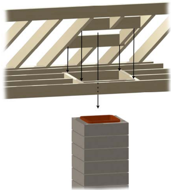
Figure 23. Roof Penetration
