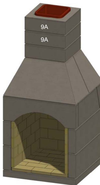
Figure 21. Chimney Complete
