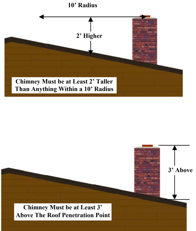
Figure 25. Chimney Height
