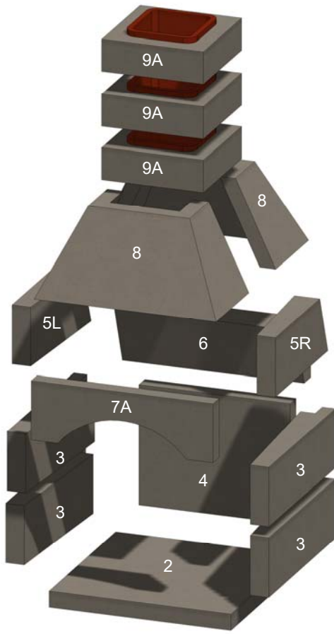
Figure 2. Fireplace Components
