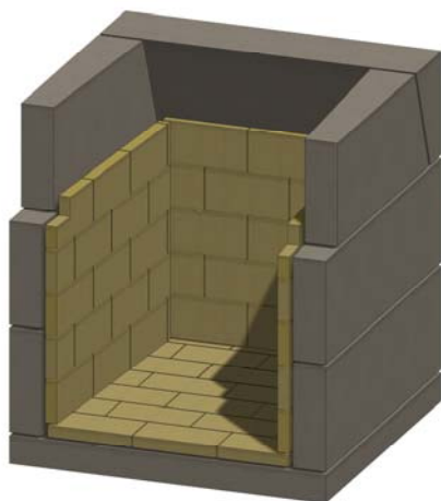
Figure 17. Sidewall Firebrick
