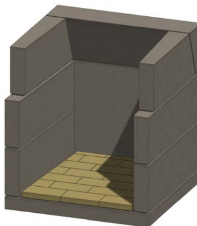
Figure 15. Floor Firebrick
