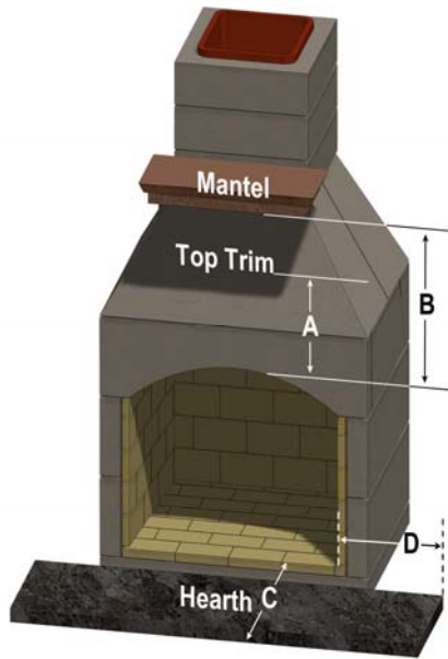
Figure 3. Clearances (Use with Table 2)
