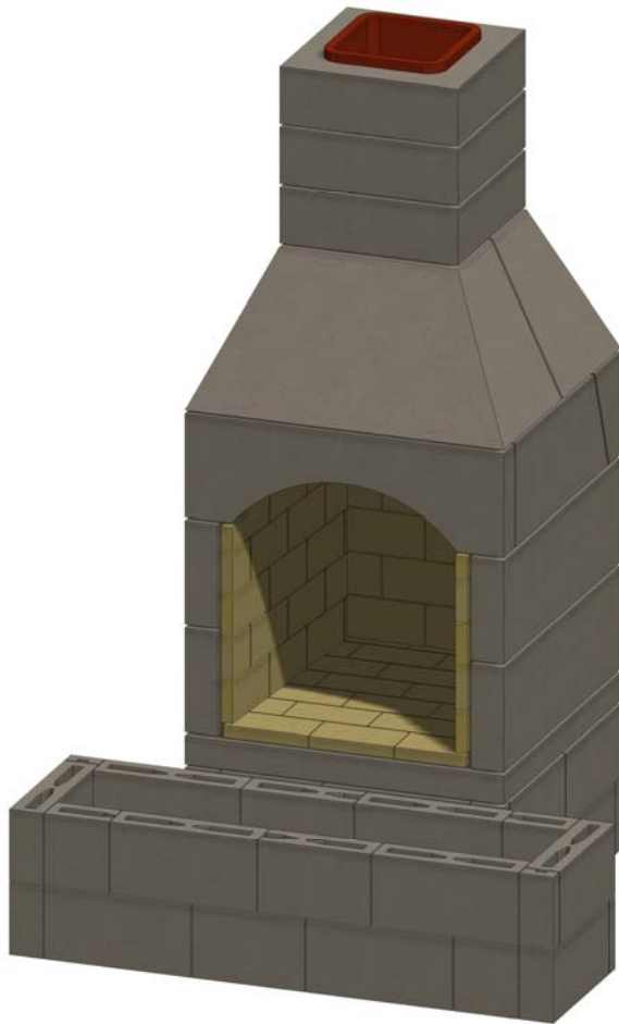
Figure 22. Hearth Base
