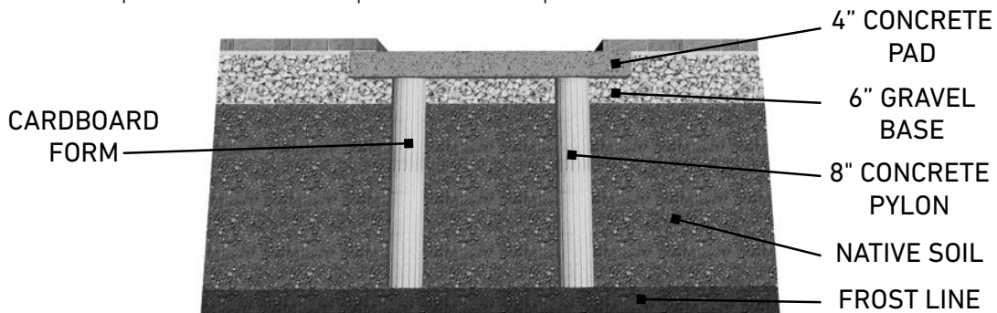
FIGURE C - Sample side view of completed concrete pad.
